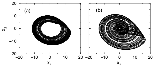
FIG. 1. Chaotic attractors of Rössler system with different parameters (a) a=0.15 and (b) a=0.25 .
